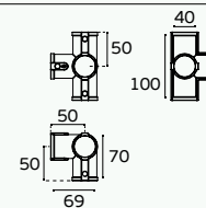
IN.09.011.TG União / Union / Unión
