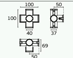
IN.09.012.TG União / Union / Unión
