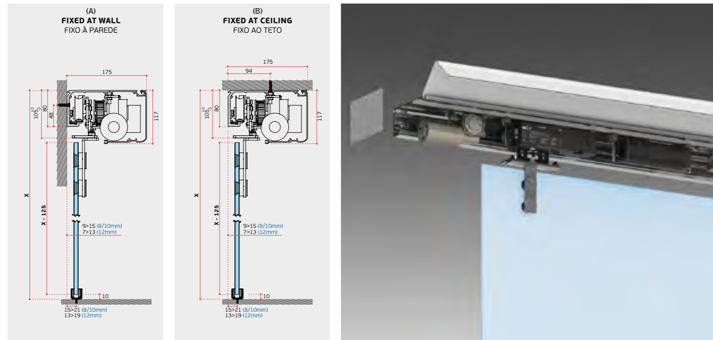
(B) FIXED AT CEILING / FIXO NO TETO
