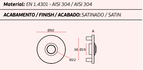
IN.24.207 Interruptor / Switch / Interruptor. MÁX: 12 VOLTS
