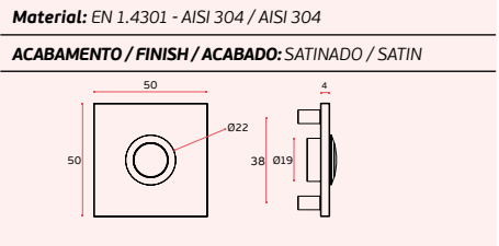
IN.24.204 Interruptor / Switch / Interruptor. MÁX: 12 VOLTS
