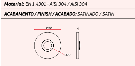
IN.24.203 Interruptor / Switch / Interruptor. MÁX: 12 VOLTS
