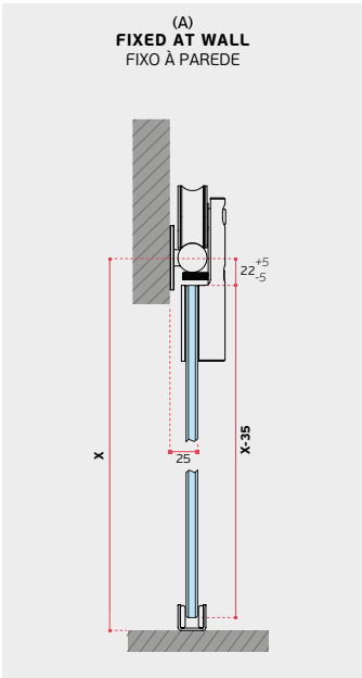
(A) FIXO À PAREDE / FIXED TO THE WALL/ FIJADO A LA PARED
