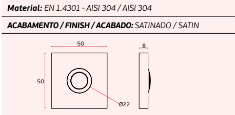
IN.24.201 Interruptor / Switch / Interruptor. MÁX: 12 VOLTS
