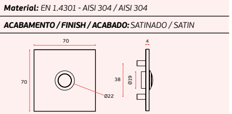
IN.24.205 Interruptor / Switch / Interruptor. MÁX: 12 VOLTS
