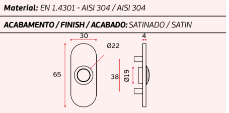
IN.24.209 Interruptor / Switch / Interruptor. MÁX: 12 VOLTS
