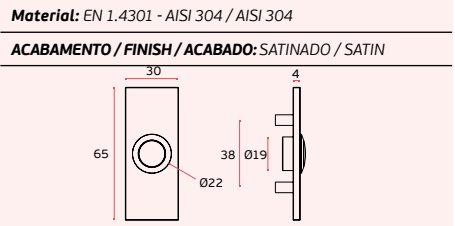
IN.24.206 Interruptor / Switch / Interruptor. MÁX: 12 VOLTS
