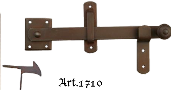
Art.1710 Saltarello/Thumblatch Asta/Bar: 250 mm Placca/Backplate: 260X40mm
